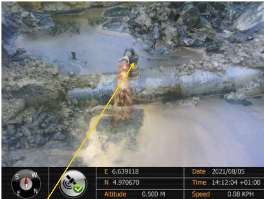
Close-up: 3" ball valve with 2" extension pipe installed at 12 o'clock position on 20" Kolocreek Pipeline at Okporowo. Picture was taken during Joint Investigation of 5 th August 2021.
