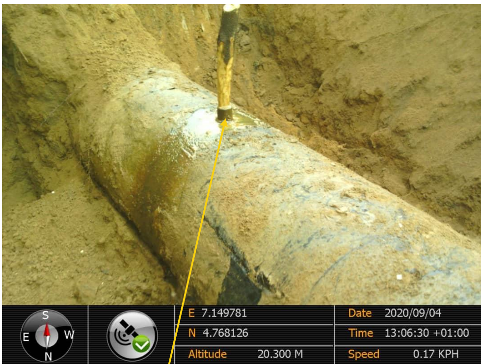
Close-up: Plugged crude oil theft point installed at 12 o'clock position on 28" Nkpoku - Bomu Pipeline at Ejamah . Picture was taken during Joint Investigation on 4th September 2020.
