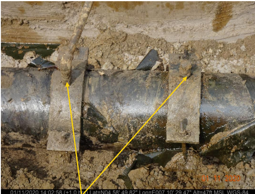
Close-up: 2nos crude oil theft points installed at 12 o'clock position on 12" Imo River2 - Ogale Pipeline at Igiriukwu isietitioha Owaza . Picture was taken during Joint Investigation on 1st November 2020.
