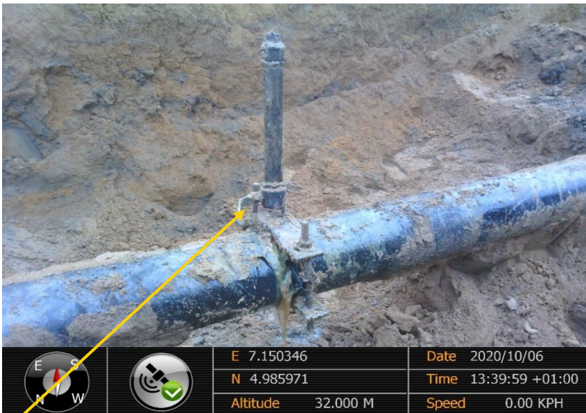
Close-up: 1.5'' locally fabricated clamp with 1.5'' valve installed at 12 o'clock position on 8'' Nkali ImoRiver2 Pipeline at Nkali. Picture was taken during Joint Investigation on 6th October 2020.
