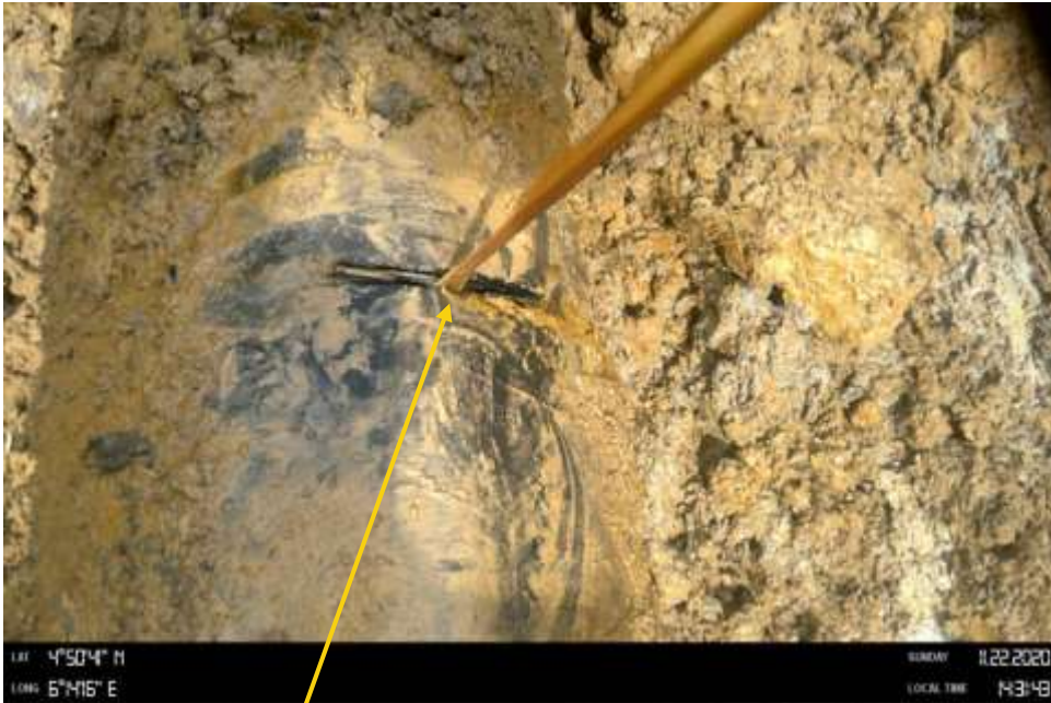
Close-up : Point 2: 2nos hacksaw cut 75m apart at 12 o'clock on 16inch NunRiver – Kolocreek Pipeline at Otugwe. Picture was taken during Joint Investigation on 22nd November 2020.
