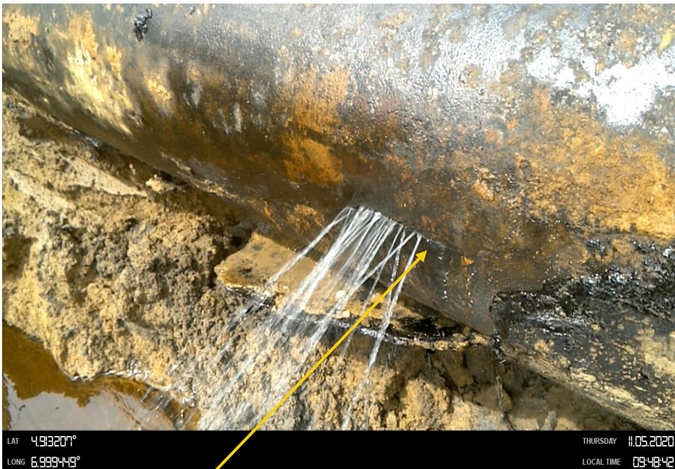
Close-up: Inward dent / Tear at 9 o'clock position on 8" Agbada 2 - Nkpoku Pipeline at Rukpokwu . Picture was taken during Joint Investigation on 5th November 2020.
