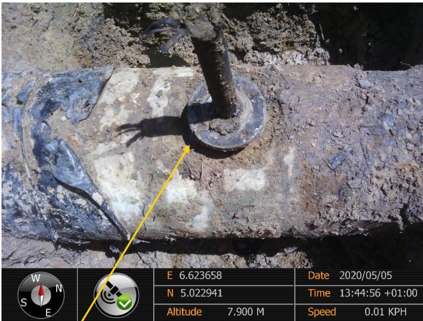
Close-up: 3" welded flange installed at 12 o'clock position on 14" Okordia Rumuekpe Pipeline at Edeoha. Picture was taken during Joint Investigation of 5th May 2020.
