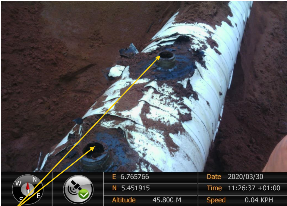
Close-up: 2nos 2" nipple (0.5m apart) installed at 12 o'clock position on 16" Egbema - Assa Pipeline at Umudike. Picture was taken during Joint Investigation of 30 th March 2020.
