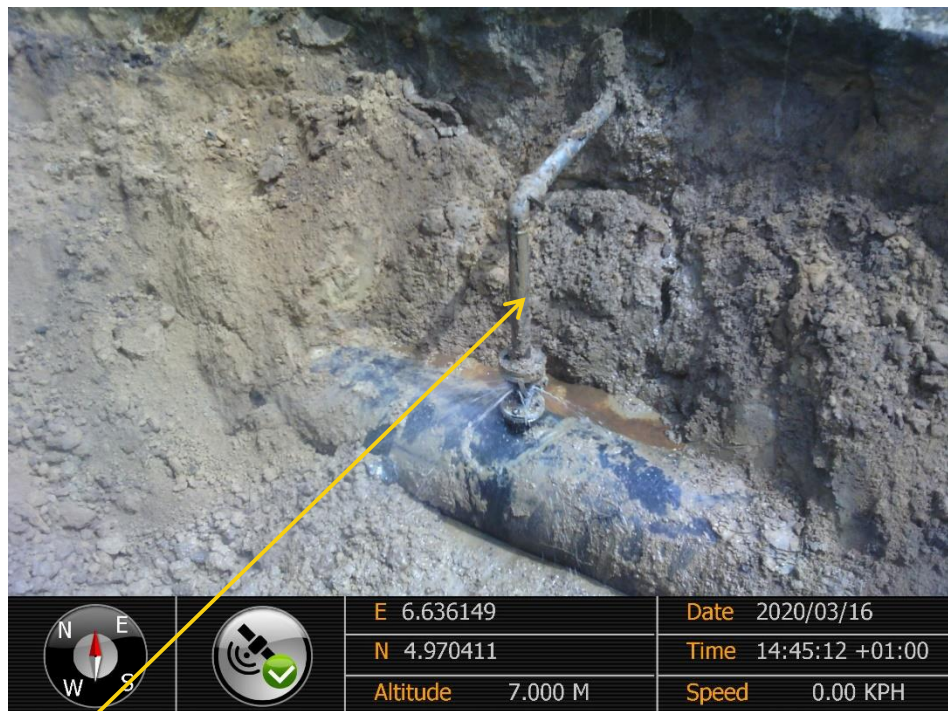
Close-up: 2" valve installed at 12 o'clock position showing water and oil on 20" Kolocreek Pipeline at Okporowo. Picture was taken during Joint Investigation of 16 th March 2020.
