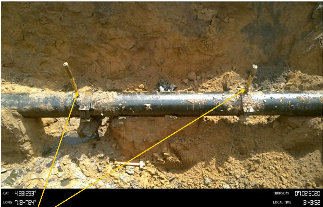
Close-up: plugged 2 nos 2inch Bulb valves installed at 12 o'clock position on 12" ImoRiver 2 – Ogale Pipeline at Okohia. Picture was taken during Joint Investigation 2nd July 2020.
