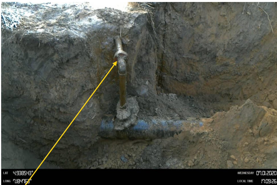
Close-up: 3" ball valve installed with elbow at 12 o'clock to 3 o'clock position on 12" Imo River - Ogale Pipeline at Umulolo. Picture was taken during Joint Investigation 1st July 2020.
