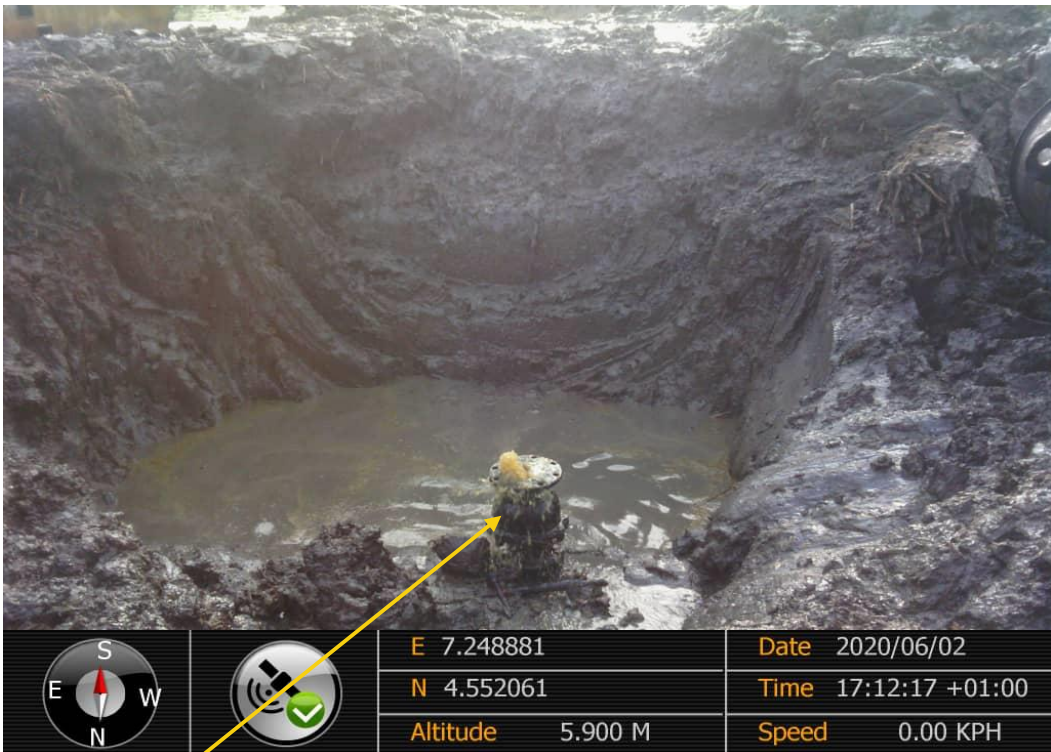
Close-up: 6" Full ball valve installed at 12 o'clock position on 28" Bomu - Bonny Pipeline at Owokiri . Picture was taken during Joint Investigation 2nd June 2020.
