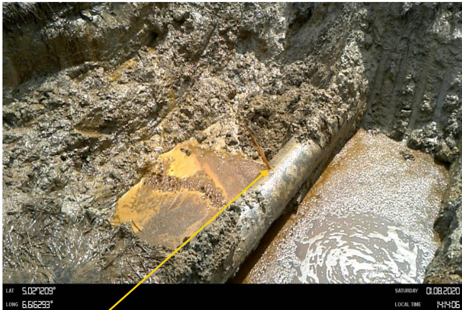
Close-up: 15mm drilled hole installed at 12:15 o'clock position on 14" Okordia - Rumuekpe Pipeline at Edeoha. Picture was taken during Joint Investigation of 1 st Aug 2020.
