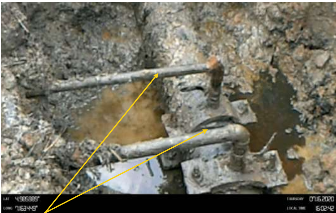
Close-up: 2nos of 1.5inches and 1inch ball valves installed at 12 o'clock position on 8" Nkali Ogale Pipeline at Odagwa. Picture was taken during Joint Investigation 16th July 2020.
