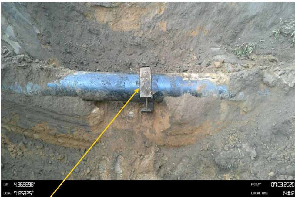
Overview: Part of spill impact on 12" ImoRiver 1 – Ogale Pipeline at Umulolo. Picture was taken during Joint Investigation 3rd July 2020.
