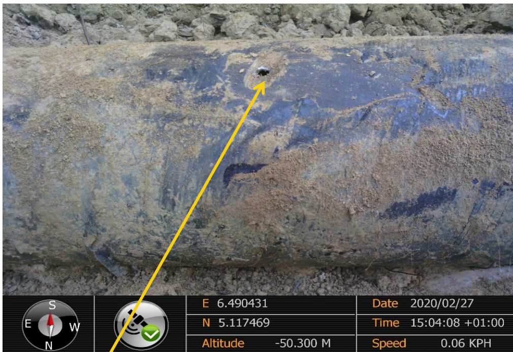
Close-up: 10mm Drilled hole on 14" Okordia Rumuekpe Pipeline at Akalamini. Picture was taken during Joint Investigation of 27 th February 2020.
