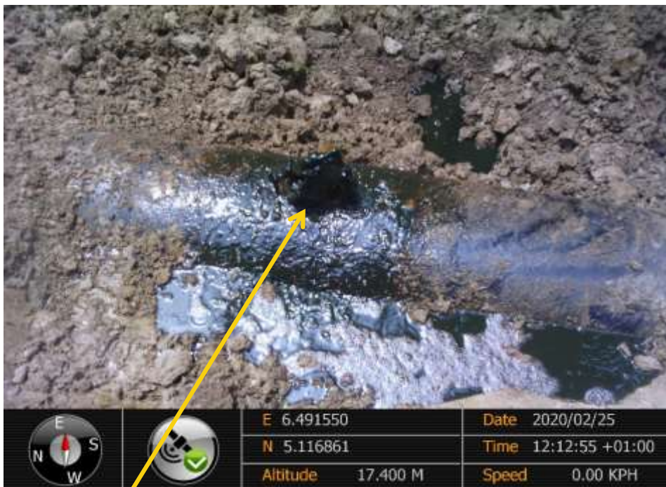
Close-up: Point 5 drilled hole at 12 o'clock position on 14" Okordia Rumuekpe Pipeline at Akalamini. Picture was taken during Joint Investigation of 25 th February 2020.
