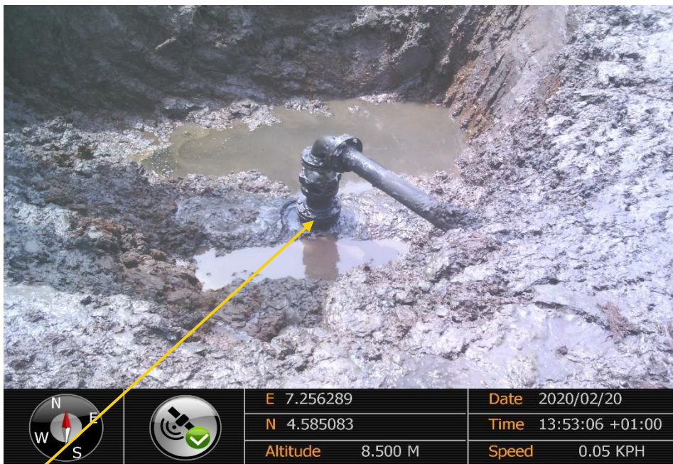
Close-up: 4" Valve installed at 12 o'clock position on 28" Bomu - Bonny Pipeline at Bodo West. Picture was taken during Joint Investigation of 20 th February 2020.
