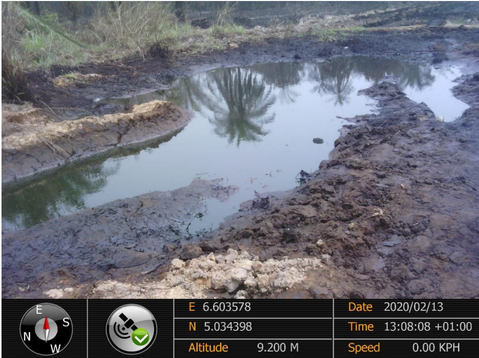
Overview: Part of spill impact on 14" Okordia - Rumuekpe Pipeline at Ikata. Picture was taken during Joint Investigation of 13 th February 2020.
