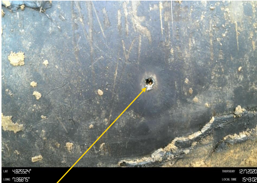
Close-up 2: 4 nos 5mm drilled hole at 2 o'clock position on 36inch Nkpoku Ogale Pipeline at Agbonchia. Picture was taken during Joint Investigation on 17th Dec 2020.
