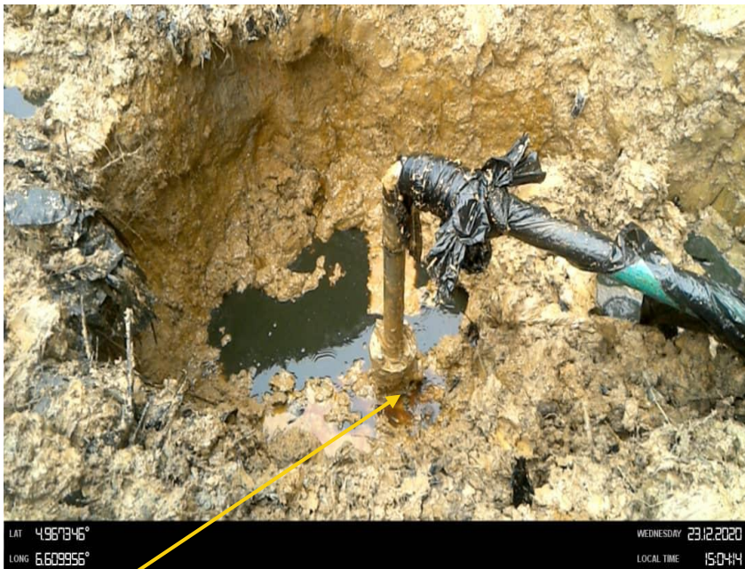
Close-up: 2'' valve installed at 12 o'clock position connected to a 2'' galvanized pipe on 20'' Kolocreek Rumuekpe Pipeine at Owerewere. Picture was taken during Joint Investigation on 23rd Dec 2020.
