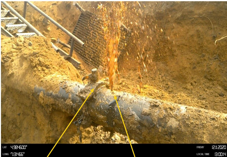
Close-up: 1 inch ball valve illegal connection and drilled hole installed at 12 o'clock position on 8'' Nkali – Imo River2 Pipeline at Odagwa. Picture was taken during Joint Investigation on 11th December 2020.
