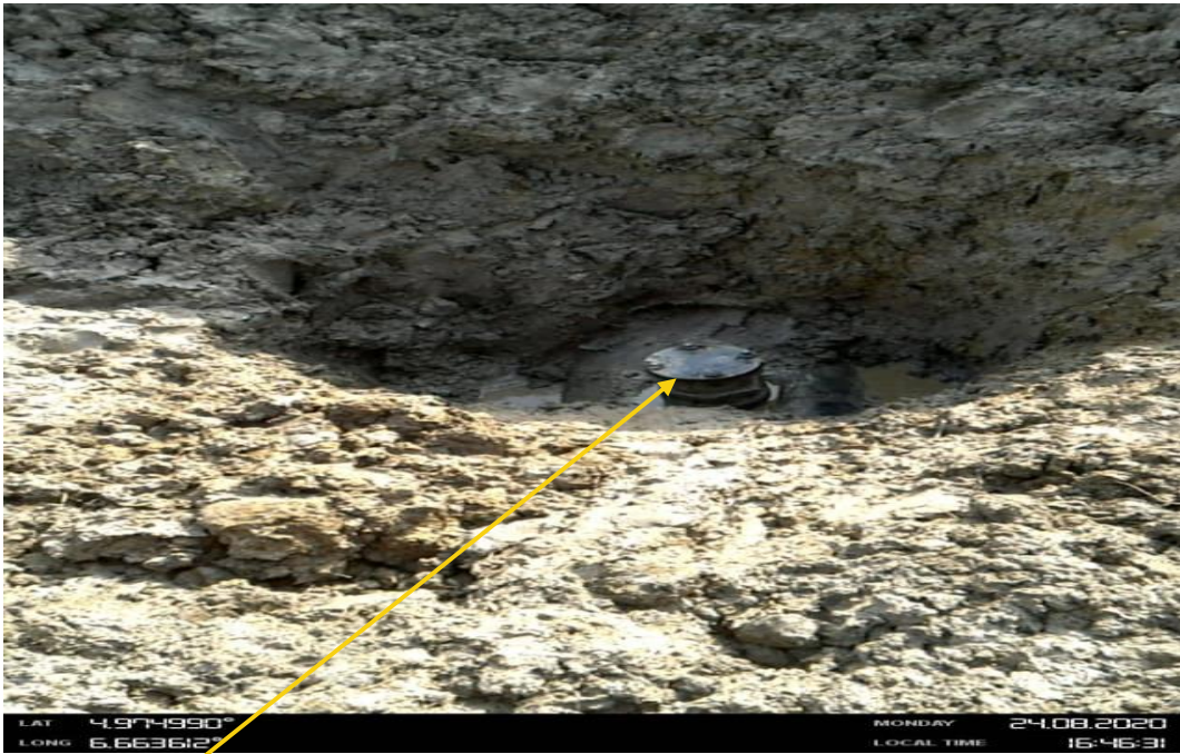
Overview: Part of spill impact on 20" Kolocreek – Rumuekpe Pipeline at Ihunwo. Picture was taken during Joint Investigation on 24th August 2020.
