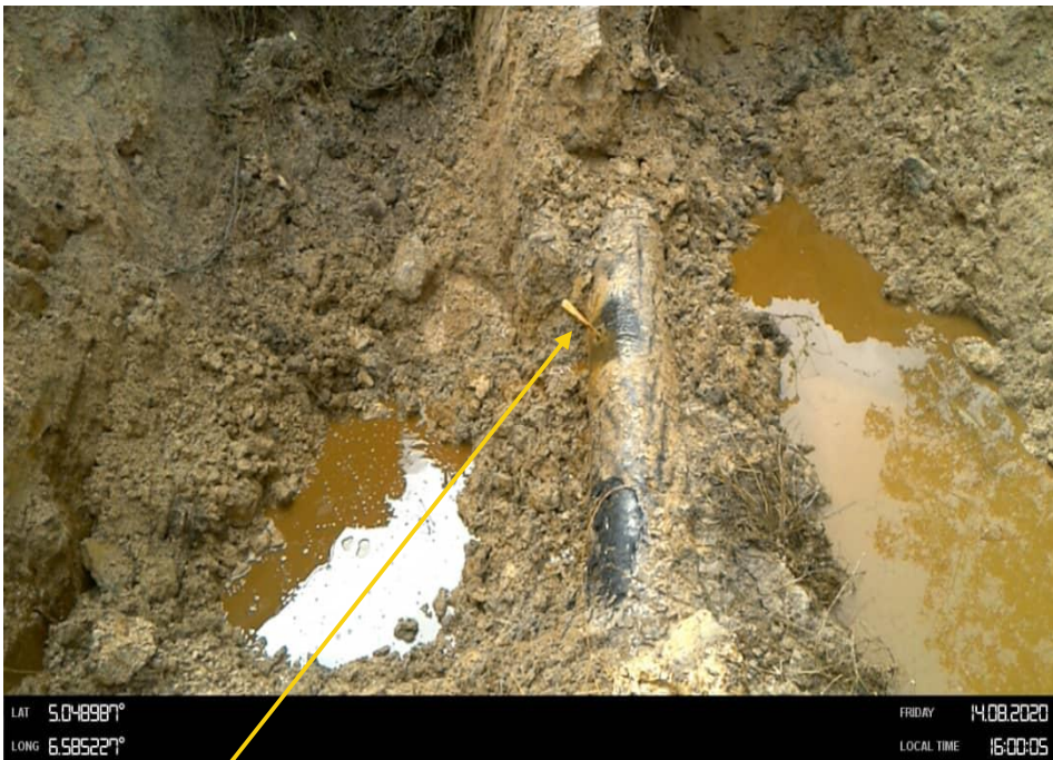
Close-up: 12mm smooth round-edge hole installed at 1 o'clock position on 14" Okordia Rumuekpe Pipeline at Ula-lkata. Picture was taken during Joint Investigation 14th August 2020.
