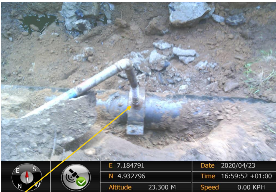
Close-up: 1 1/2" Locally fabricated clamped installation with an elbow at 12 o'clock on 12" Imo River 1- Ogale Pipeline at Etituzo-Umuololo . Picture was taken during Joint Investigation of 23 rd April 2020.
