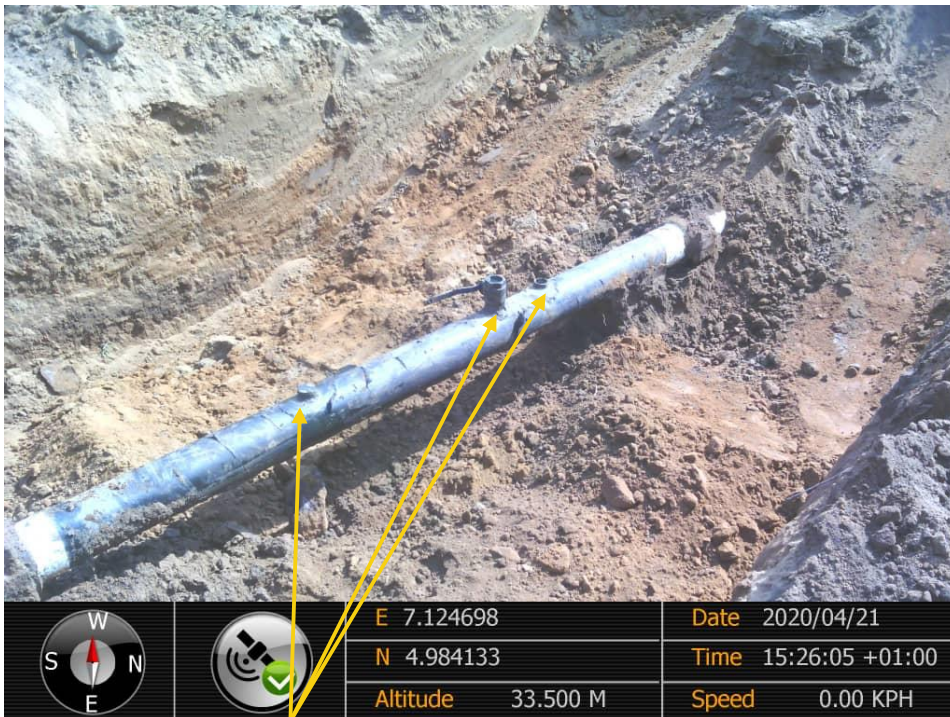
Close-up: 3Nos crude oil theft points installed at 12 o'clock position on 8" Nkali – Imo River2 Pipeline at Odagwa. Picture was taken during Joint Investigation 21st April 2020.
