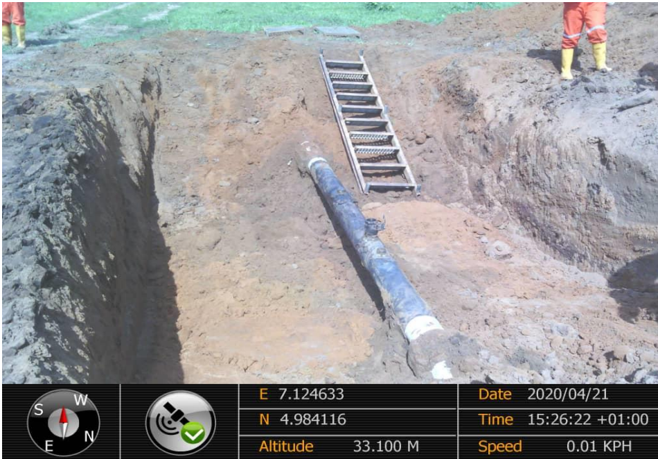
Overview: Part of spill impact on 8" Nkali – Imo River2 Pipeline at Odagwa. Picture was taken during Joint Investigation 21st April 2020.
