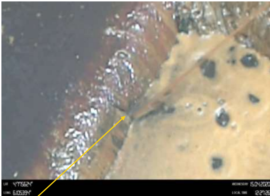
Close-up: 12mm Hacksaw cut at 11 o'clock position on 10" Diebu Creek Nun-River Pipeline at Osokama-Oporoma. Picture was taken during Joint Investigation of 15 th April 2020.
