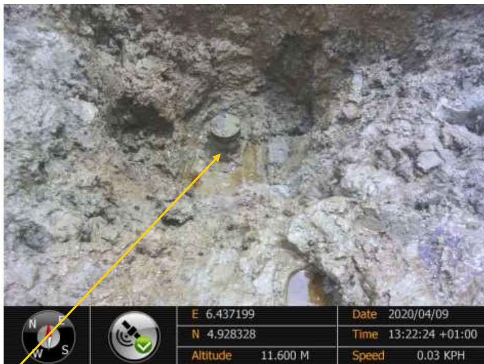
Close-up: 3" ball valve flange installed at 12 o'clock position on 20" Kolocreek-Rumuekpe Pipeline at Odau-KP9. Picture was taken during Joint Investigation of 9 th April 2020.
