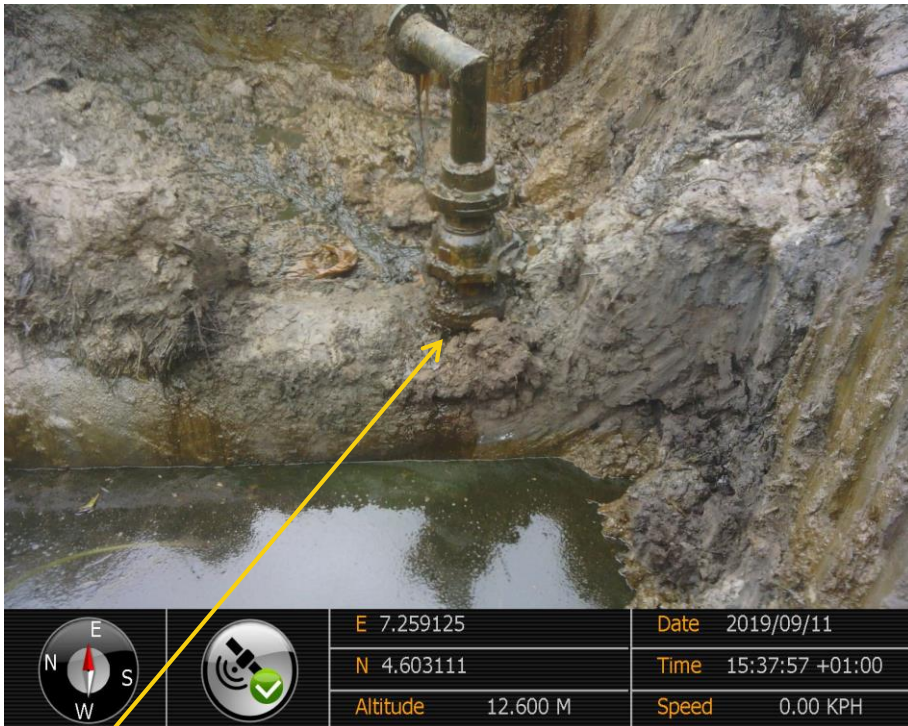
Close-up: Illegal fitting on 24" Bomu - Bonny Pipeline Right of Way at Patrick Waterside_Bodo West. . Picture was taken during Joint Investigation of 11 th September 2019.
