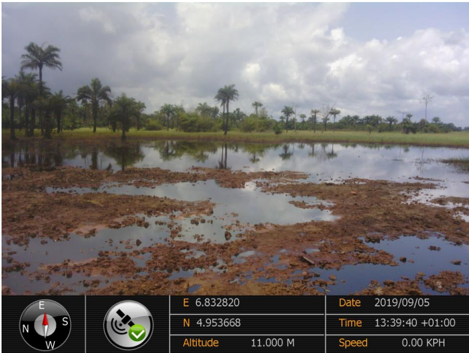
Overview: Part of spill impact on 20'' Rumuekpe - Nkpoku Pipeline Right of Way at Sime. Picture was taken during Joint Investigation of 5 th September 2019.
