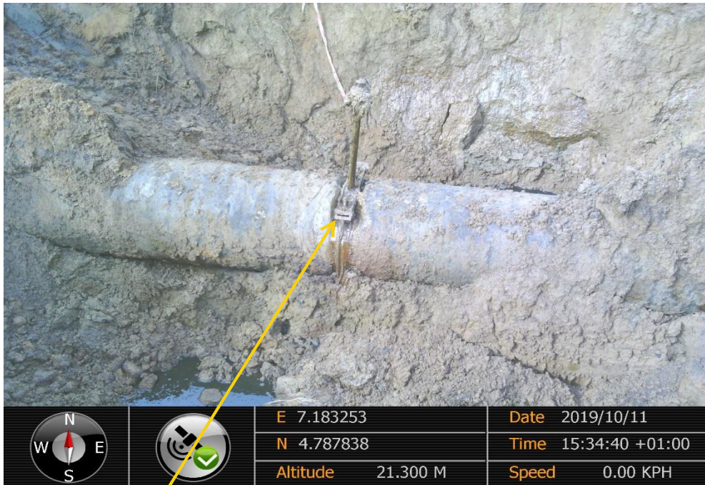
Close-up: Illegal fitting on 24" Nkpoku - Bomu Pipeline at Egbalor. Picture was taken during Joint Investigation of 11 th October 2019.
