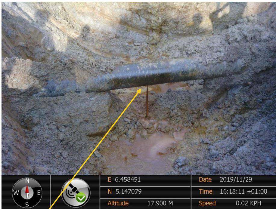
Close-up: Decoated portion of pipe on 14inch Okordia Rumuekpe Pipeline at Ikarama. Picture was taken during Joint Investigation of 29 th November 2019.
