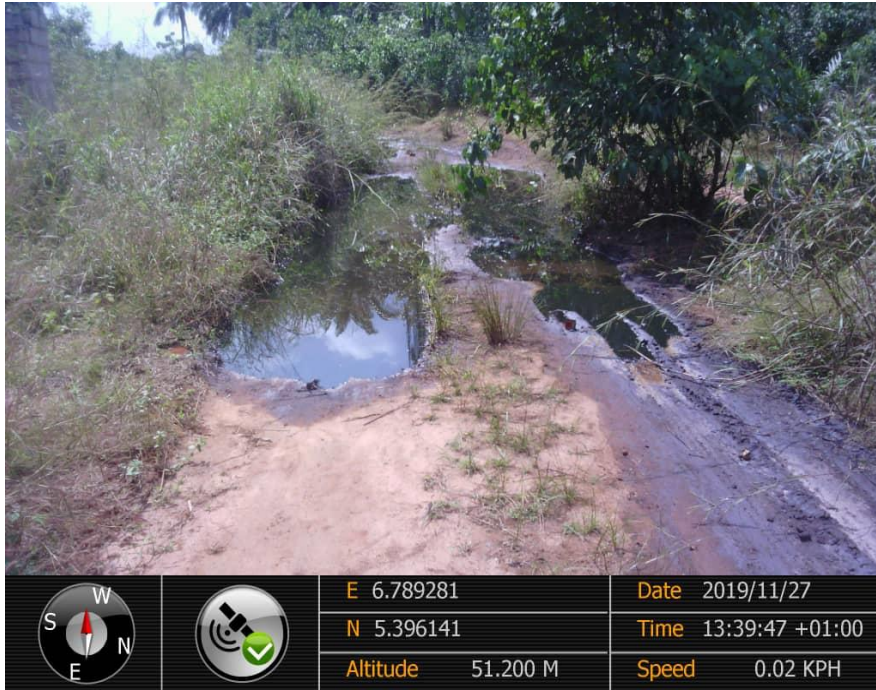
Overview: Part of spill impact on 16'' Egbema – Assa Pipeline Right of Way at Obile. Picture was taken during Joint Investigation of 27 th November 2019.
