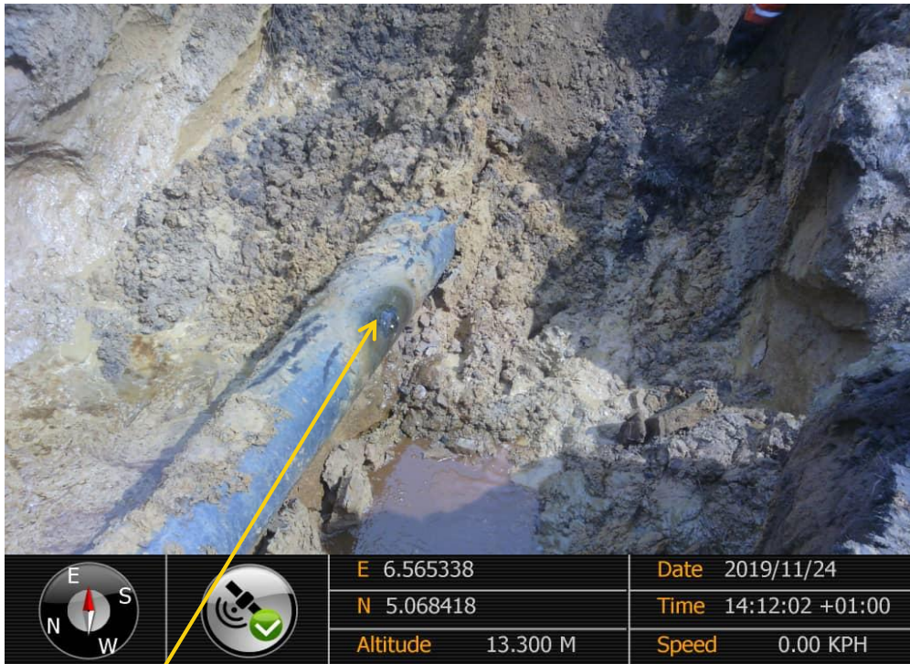
Close-up: Drilled Hole on 14" Okordia – Rumuekpe Pipeline at Ula-Okobo . Picture was taken during Joint Investigation of 24 th November 2019.
