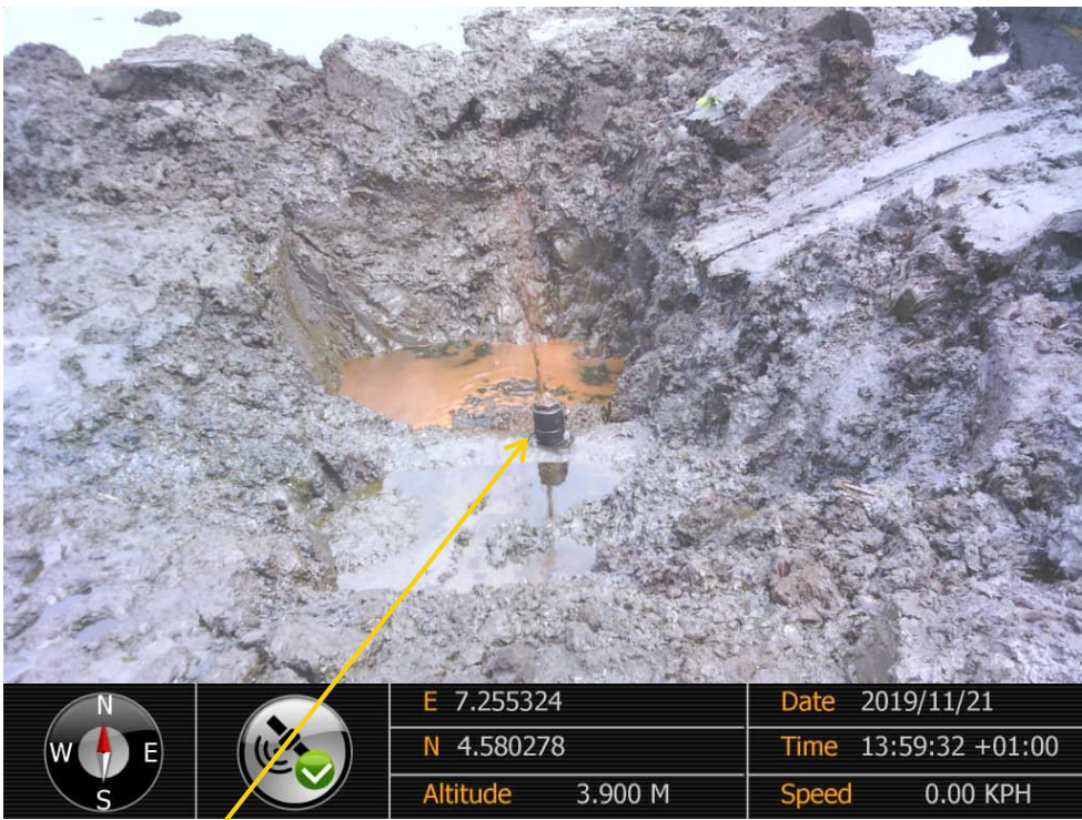
Close-up: Illegal fitting on 28" Bomu – Bonny Pipeline at Patrick Waterside - Bodo West . Picture was taken during Joint Investigation of 21 st November 2019.
