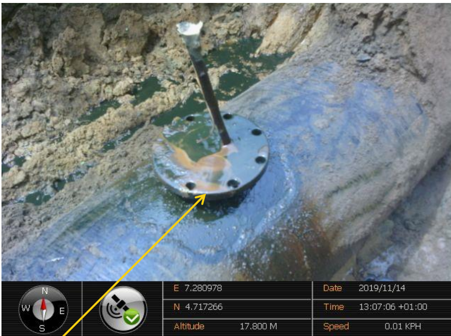
Close-up: Illegal Fitting on 24" Nkpoku - Bomu Pipeline at Kpите. Picture was taken during Joint Investigation of 14 th November 2019.
