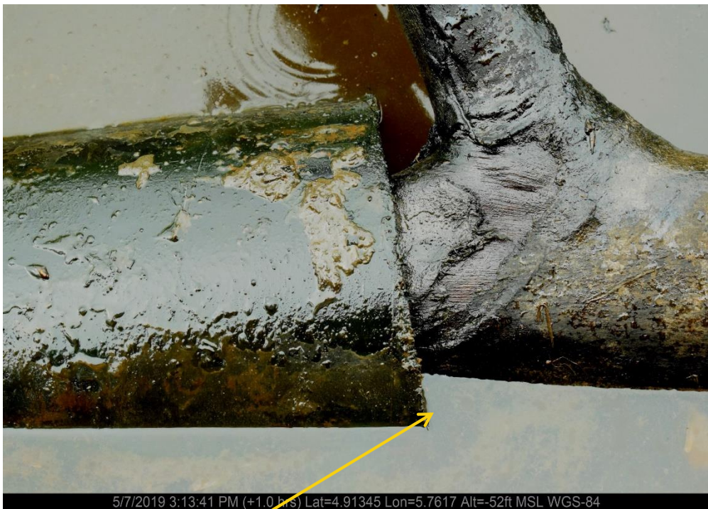
Close-up: Missing part of the Flowline on 6" Opukushi Well 25T Flowline at Egbemo-Analabiri-Agbidiana. Picture was taken during Joint Investigation of 7 th May 2019
