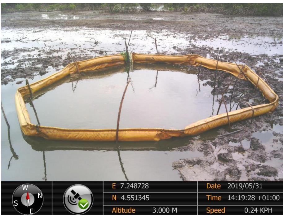
Overview: Part of spill impact on 28" Bomu – Bonny Pipeline Right of Way at Owokiri. Picture was taken during Joint Investigation of 31 st May 2019.
