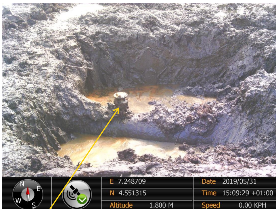
Close-up: Illegal Fitting on 28" Bomu – Bonny Pipeline at Owokiri. Picture was taken during Joint Investigation of 31 st May 2019.
