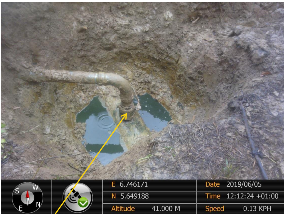
Close-up: Illegal fitting on 12'' Oguta – Egbema Pipeline at Umunkwu. Picture was taken during Joint Investigation of 5 th June 2019
