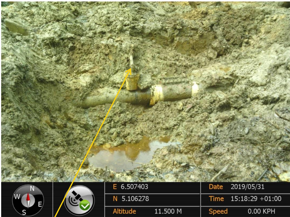
Close-up: Illegal fitting on 14" Okordia – Rumuekpe Pipeline at Oshie. Picture was taken during Joint Investigation of 31 st May 2019
