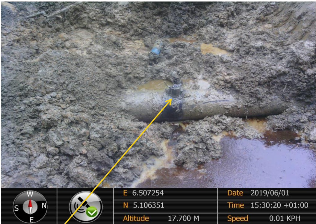
Close-up: Illegal Fitting on 14" Okordia – Rumuekpe Pipeline at Oshie. Picture was taken during Joint Investigation of 1 st June 2019.
