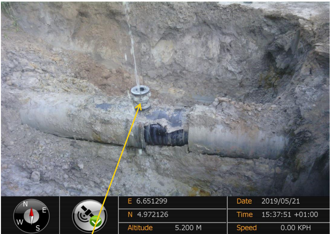
Close-up: Leaking Illegal Fitting on 20'' Kolocreek – Rumuekpe Pipeline at Okoma-1. Picture was taken during Joint Investigation of 21 st May 2019.
