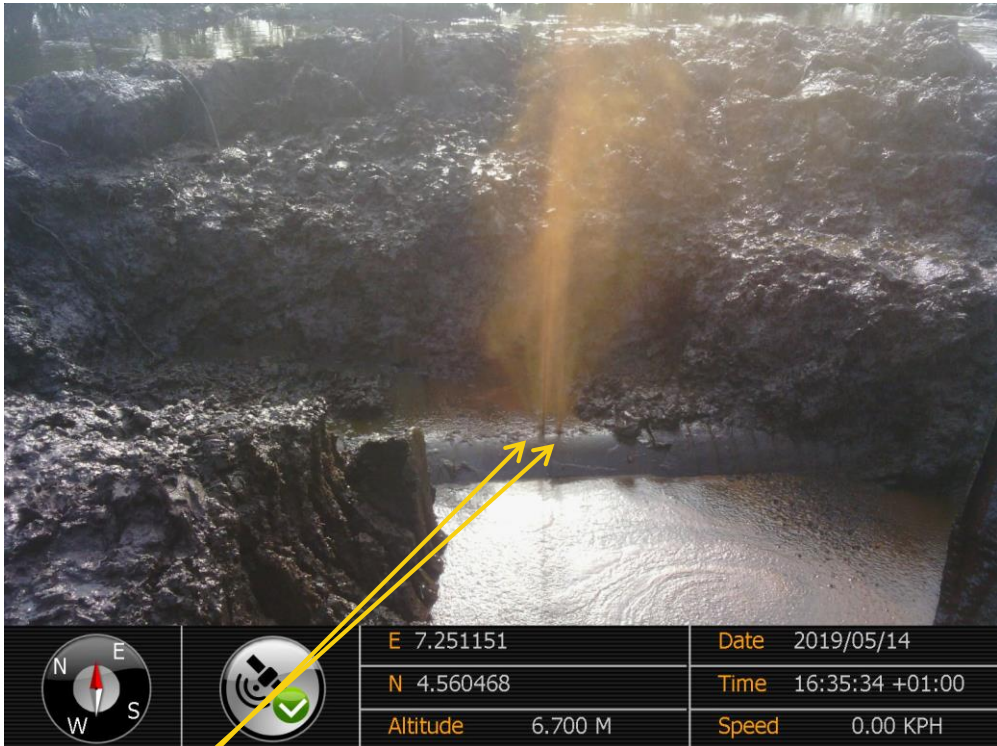
Close-up: Hack Saw Cuts on 28" Bomu – Bonny Pipeline at Owokiri. Picture was taken during Joint Investigation of 14 th May 2019
