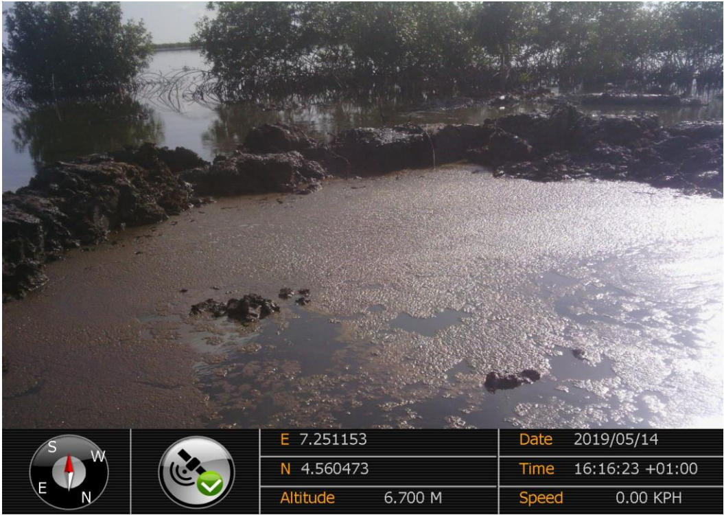
Overview: Part of spill impact on 28" Bomu – Bonny Pipeline Right of Way at Owokiri. Picture was taken during Joint Investigation of 14 th May 2019.
