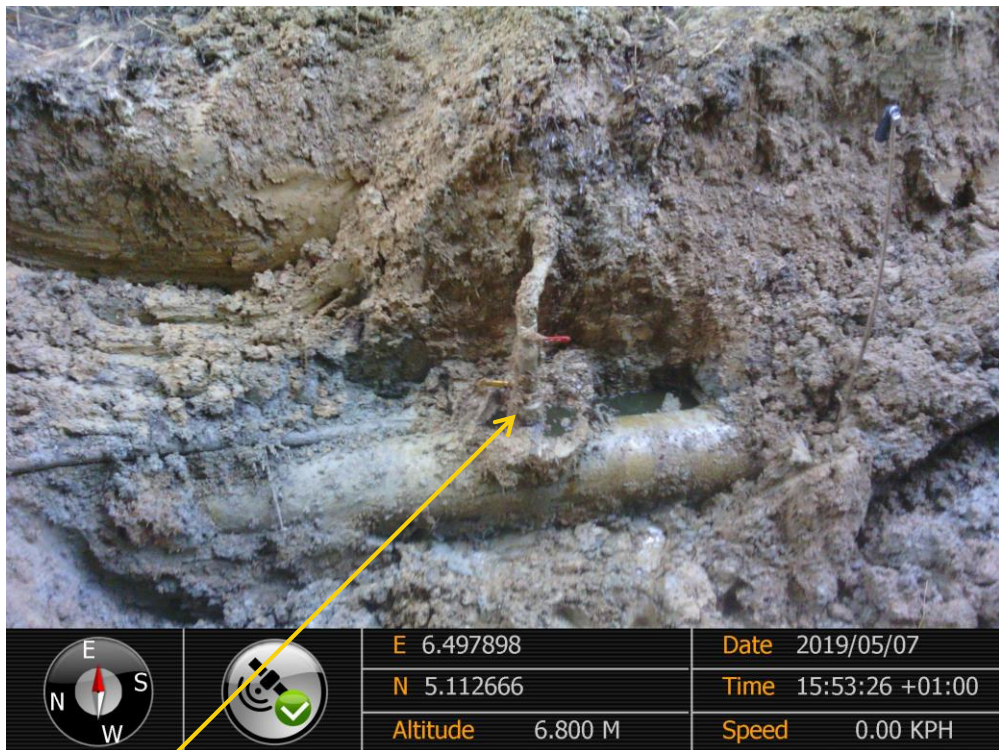
Close-up: Illegal fitting on 14" Okordia - Rumuekpe Pipeline at Akala-Olu. Picture was taken during Joint Investigation of 7 th May 2019
