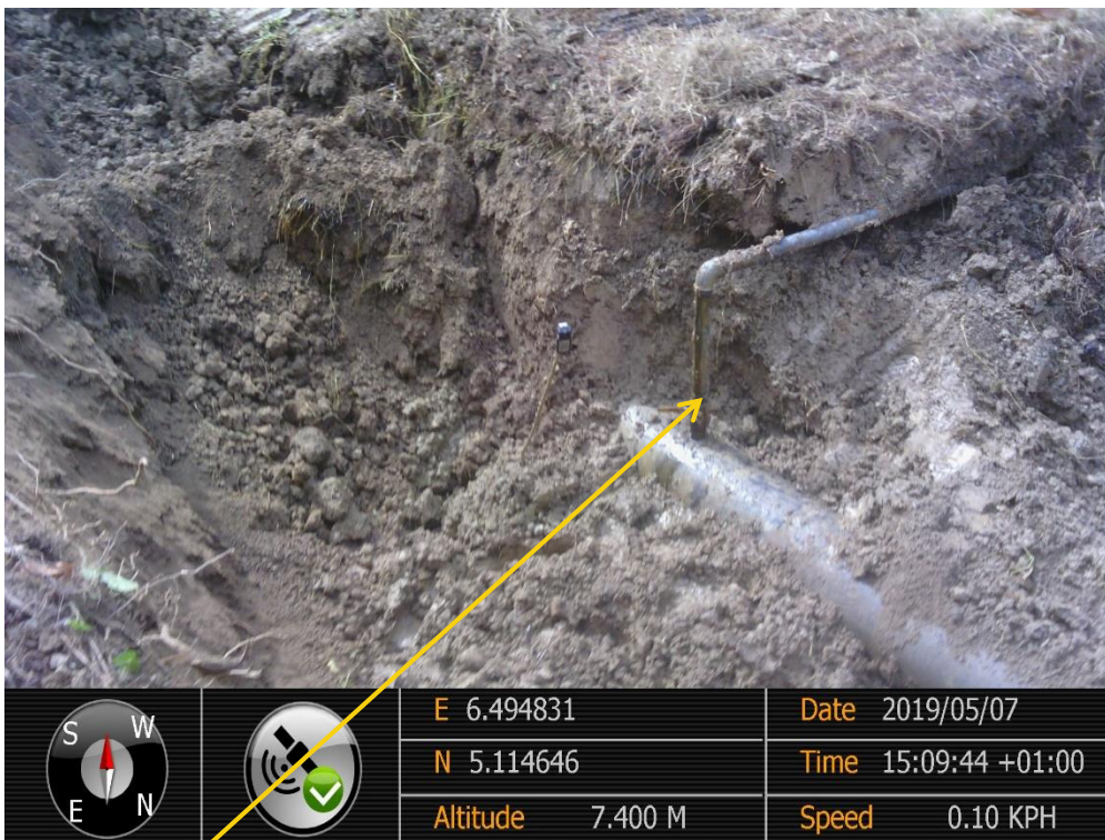
Close-up: Illegal Fitting on 14" Okordia - Rumuekpe Pipeline at Akala-Olu. Picture was taken during Joint Investigation of 7 th May 2019
