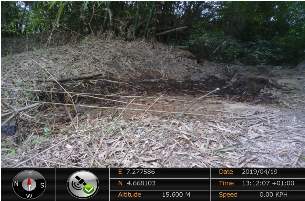
Overview: Part of spill impact on 28" Nkpoku – Bomu Pipeline Right of Way at B-Dere. Picture was taken during Joint Investigation of 19 th April 2019.
