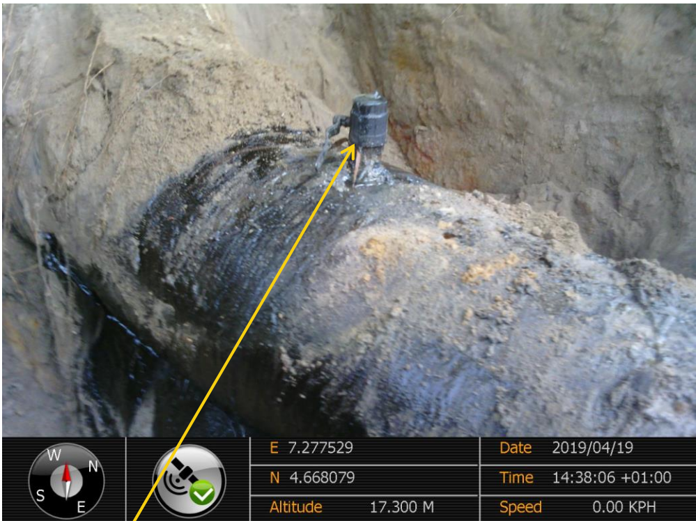
Close-up: Illegal fitting on 28" Nkpoku – Bomu Pipeline at B-Dere. Picture was taken during Joint Investigation of 19 th April 2019
