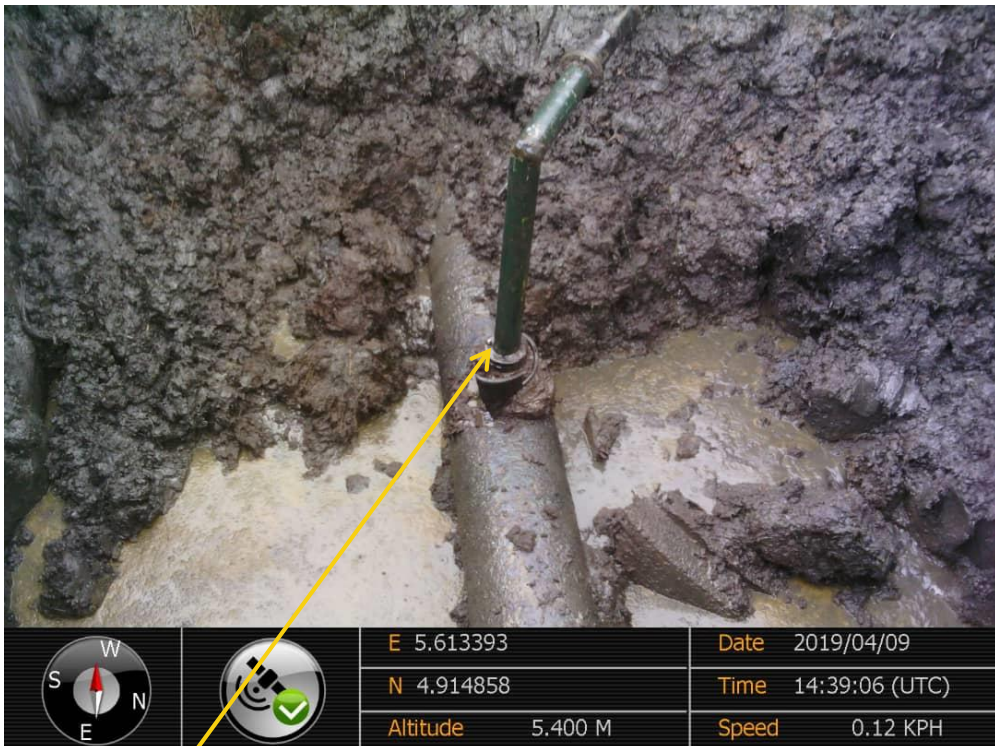
Close-up: Illegal fitting on 16'' Tunu - Brasscreek Pipeline at Agbidiana. Picture was taken during Joint Investigation of 9 th April 2019
