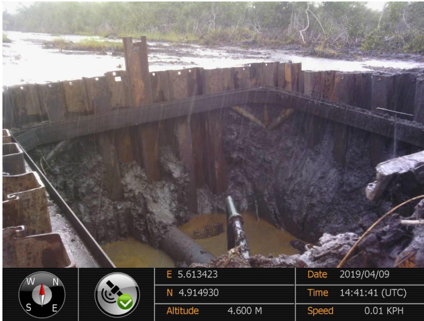
Overview: Part of spill impact on 16'' Tunu - Brasscreek Pipeline Right of Way at Agbidiana. Picture was taken during Joint Investigation of 9 th April 2019.
