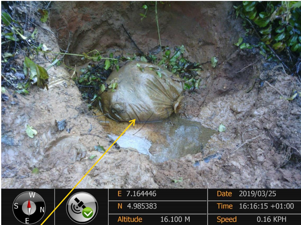
Close-up: Sand bag on 8'' Nkali - ImoRiver Pipeline at Odagwa. Picture was taken during Joint Investigation of 25 th March 2019
