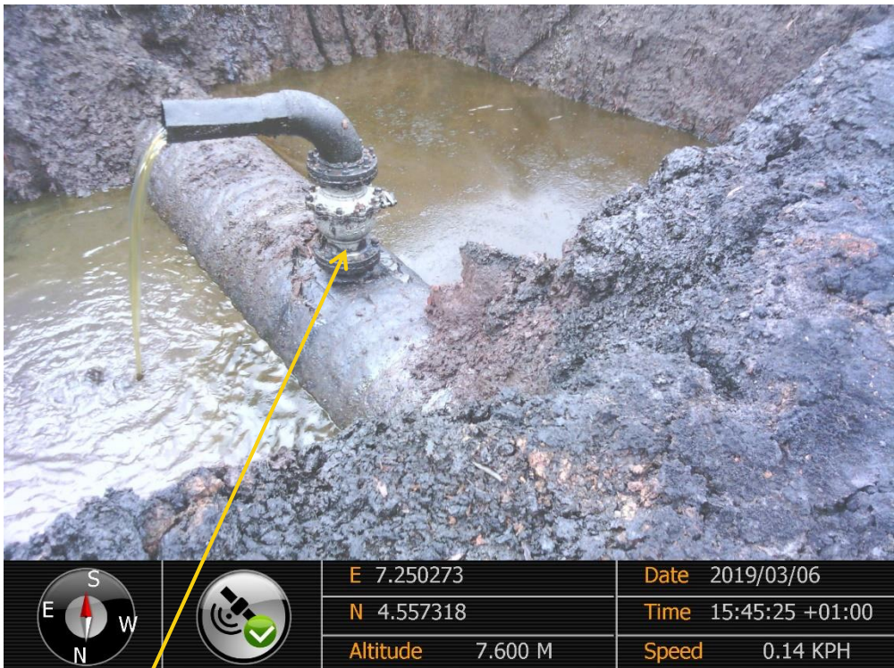
Close-up: Illegal Fitting on 28" Bomu - Bonny Pipeline at Owokiri. Picture was taken during Joint Investigation of 6 th March 2019
