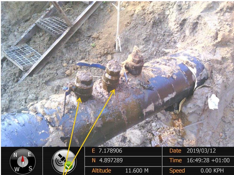
Close-up: Leaking Illegal Fittings on 12'' Imo River – Ogale Pipeline at Uzuaku. Picture was taken during Joint Investigation of 12 th March 2019
