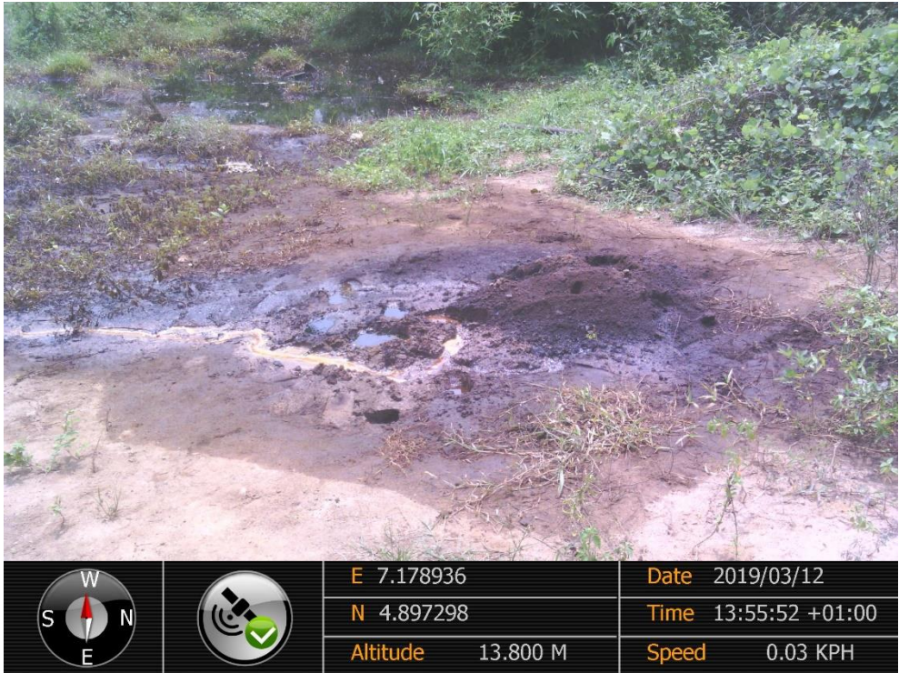
Overview: Part of spill impact on 12'' Imo River – Ogale Pipeline Right of Way at Uzuaku. Picture was taken during Joint Investigation of 12 th March 2019.
